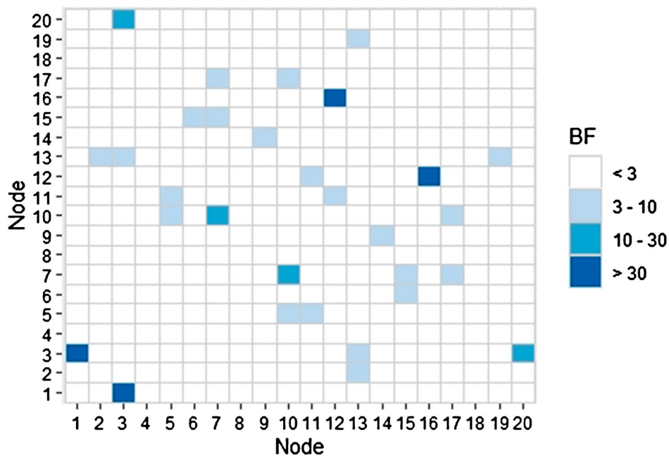
Figure 2. Bayes factors (BFs) for edge-wise group differences.
